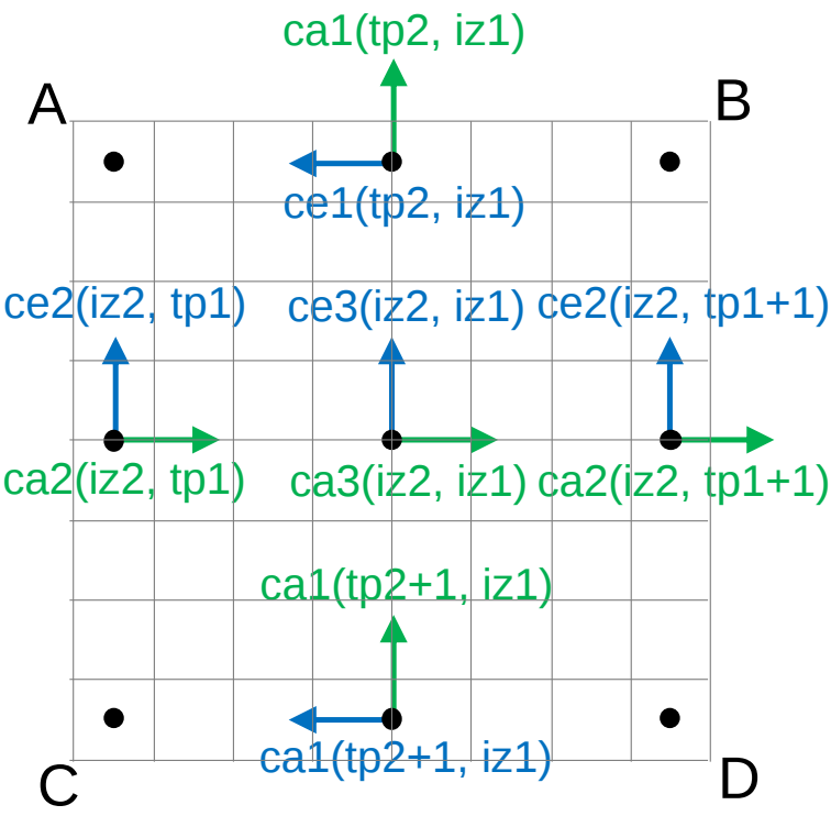
Figure J.5. The parametric representation of the interpolation coefficients cea = (ce, ca) , stored in the interpolation parameters ce1, ca1, ce2, ca2, ce3 and ca3 , is equivalent to five additional tie points for the interpolation subarea. Shown with parameter orientation and indices.
