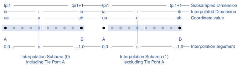
Figure 7. One-dimensional interpolation subareas, one including and one excluding tie point A.
