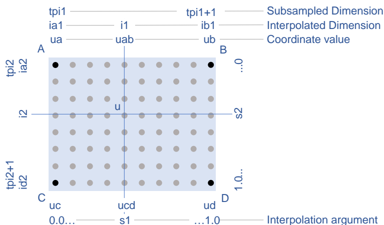
Figure 8. Two-dimensional interpolation subarea.
